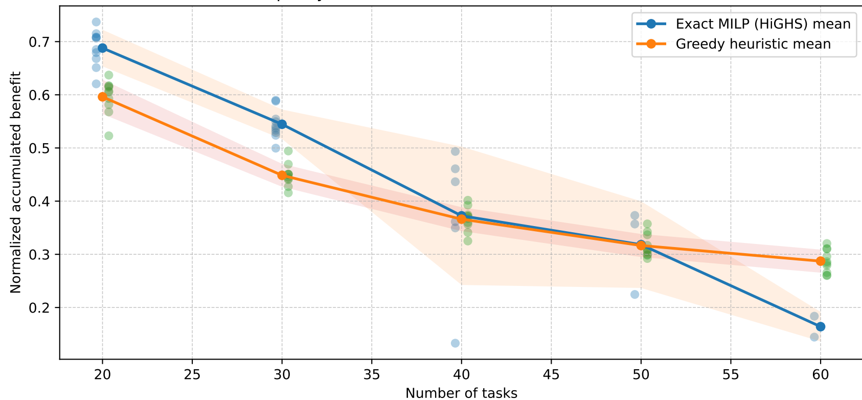
Solution quality across scaled TTAP instances - 6 Helos / 7 Areas
